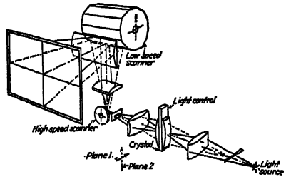
Use of cylindrical convex lenses in the Scophony television system with two motor-driven mirror wheels to provide scanning.
